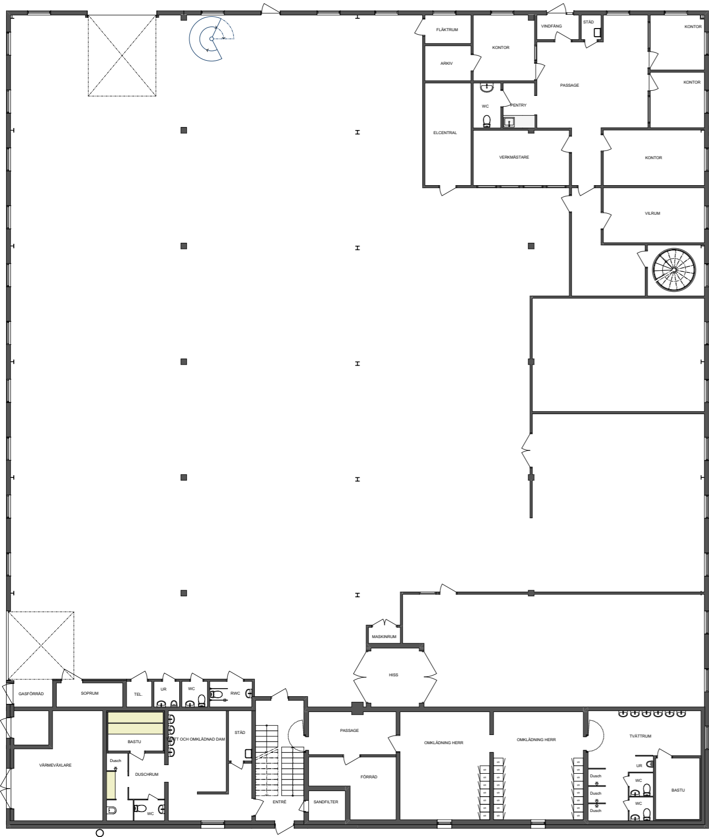
Bottenplan
